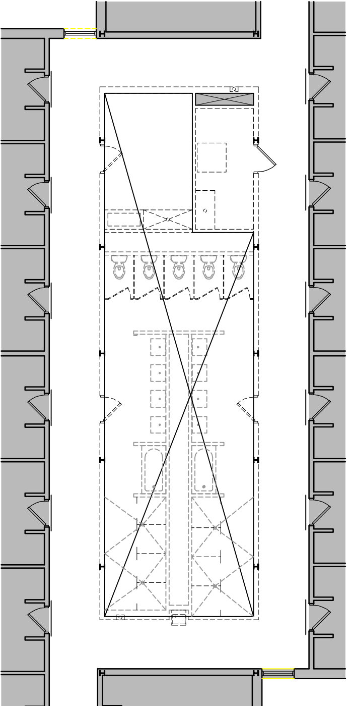
N 1/4" = 1'-0" WEST WING DEMOLITION PLAN (EAST WING SIM.) (TYP. @ FIRST, SECOND, THIRD AND FOURTH FLOORS)
