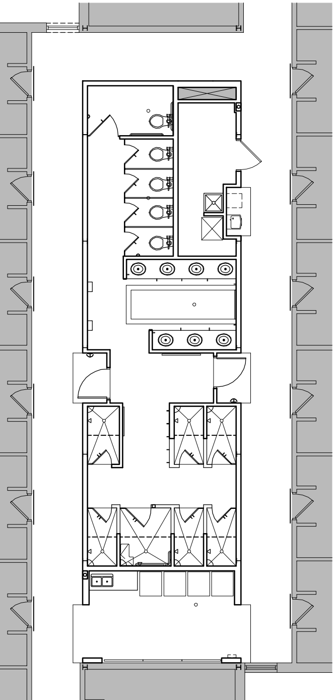
N 1/4" = 1'-0" WEST WING FLOOR PLAN (EAST WING SIM.) (TYP. @ FIRST, SECOND, THIRD AND FOURTH FLOORS)
